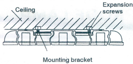
Mounting brackets ceiling mounting
