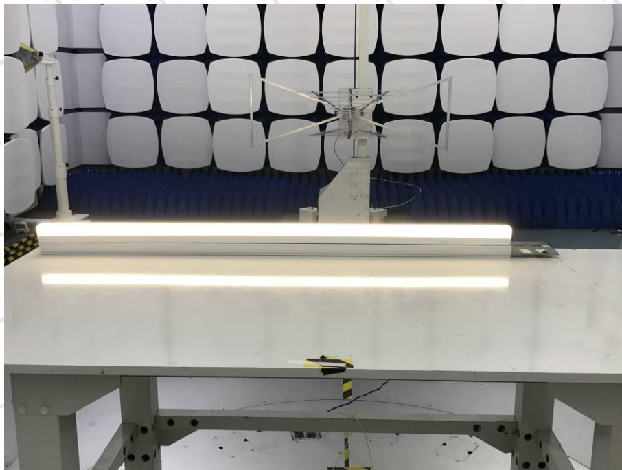
Photo10 Radiated Emission Test
