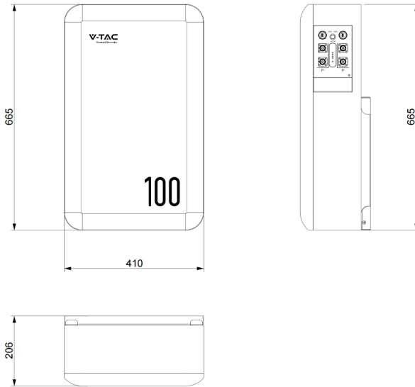
Fig. 5-1 Product Dimensions
